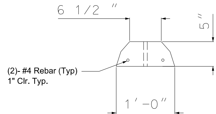
Typical Section
